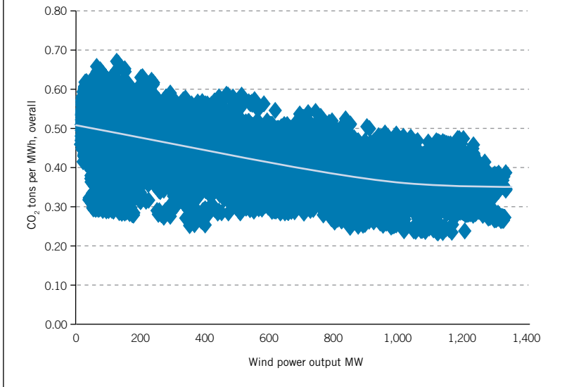
Figure 28: Irish wind power & CO 2 emissions
