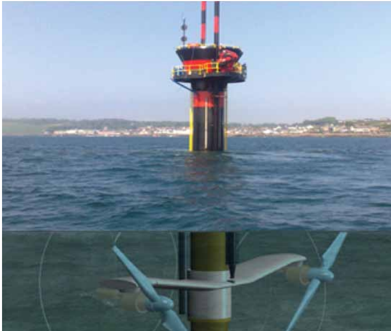
Figure 27: SeaGen at Strangford Lough
