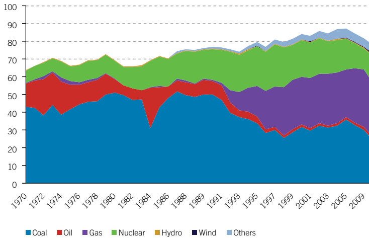
Figure 7: Fuel mix of UK power generation since 1970
